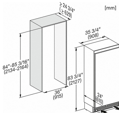
K2901Vi, K2911Vi, F2901Vi, F2911Vi, inner space, MasterCool, installation drawings
