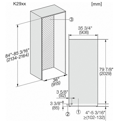
K2901Vi, K2901SF, K2911Vi, K2911SF, MasterCool, *footnote, installation drawings
