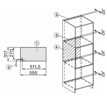
ESW7030 installation drawings
