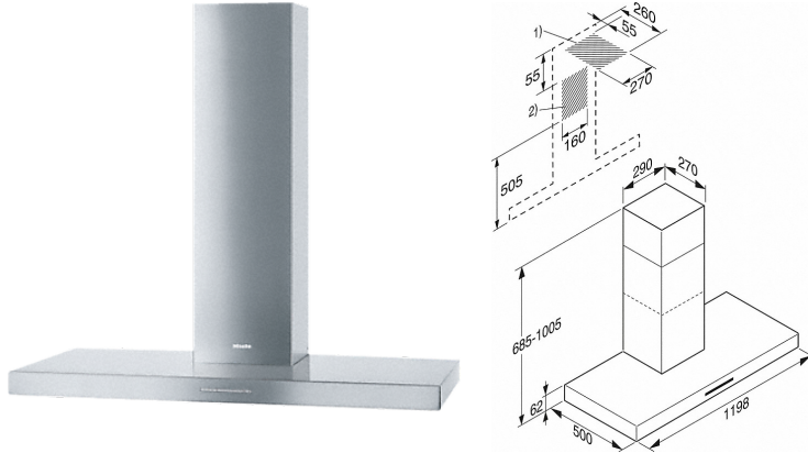
DA 4228 (Installation drawing)
